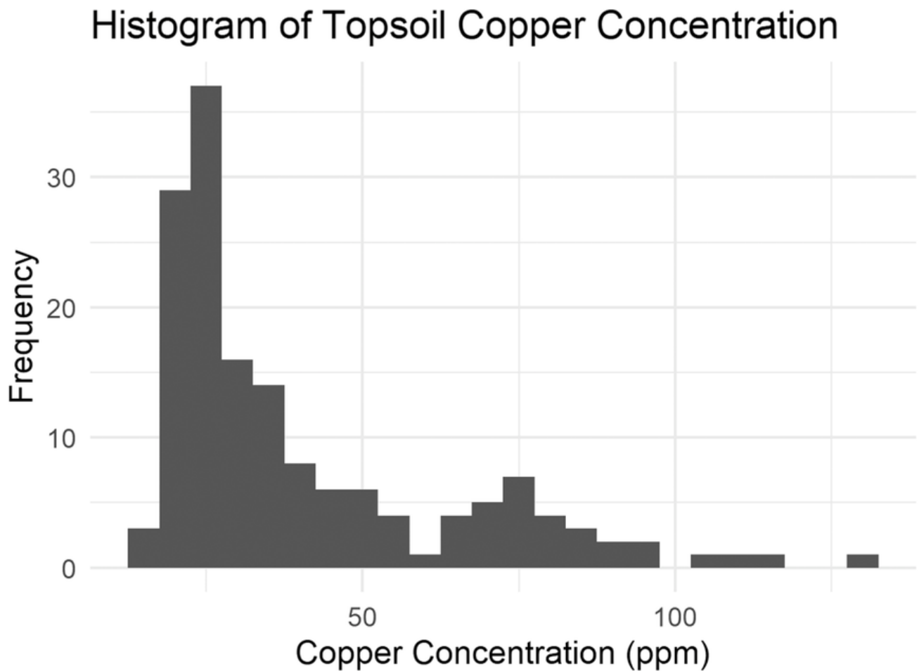
Histogram of topsoil copper concentration in parts per million.
