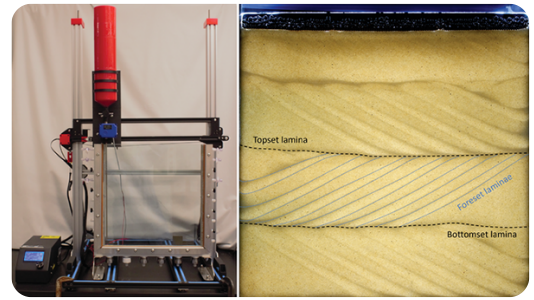
Left: A Queen's University research team modified this 3D printer so that it could dispense sand. Right: An example of a heterogeneous sand pack created by the modified 3D printer. Photos by Mitchell Davidson.
