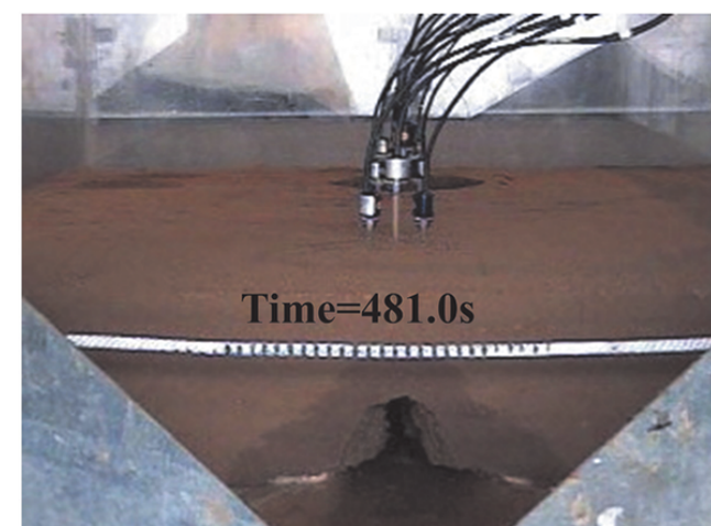
The dynamics in pipeflow and sediment concentrations are demonstrated during experiments conducted by Wilson (2011) and used by Nieber et al. (this publication) for numerical modeling of internal erosion by pipeflow. Reprinted with permission from Fig. 5 of Wilson et al. (2018).
