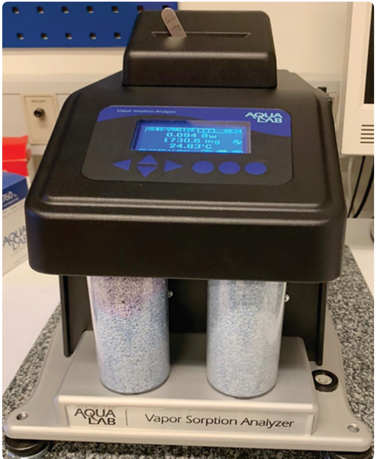
The vapor sorption analyzer provides sorption isotherm measurements by automatically wetting and drying the sample while recording the change in the sample mass. Photo by
